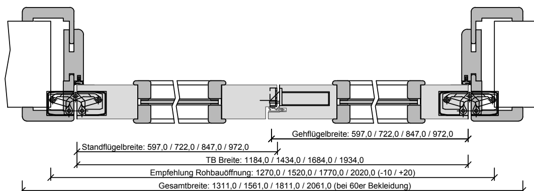
Q-FR-TB-HZ-2FLG-STU-FR-LA.dwg
