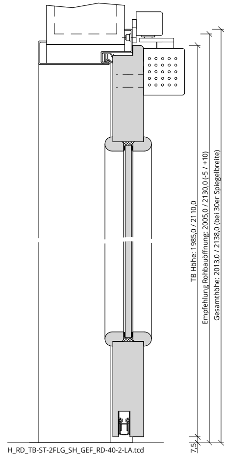
H_RD_TB-ST-2FLG_SH_GEF_RD-40-2-LA.tcd
