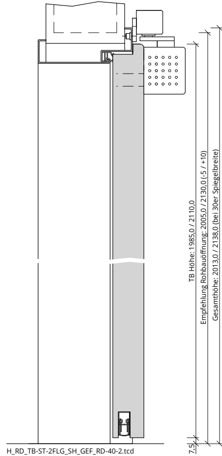
H_RD_TB-ST-2FLG_SH_GEF_RD-40-2.tcd
