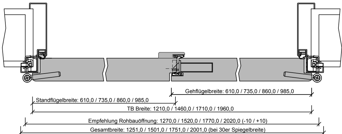
G-Q-SD-TB-SZ-2FLG-SH-GEF-SD-SSK3.dwg
