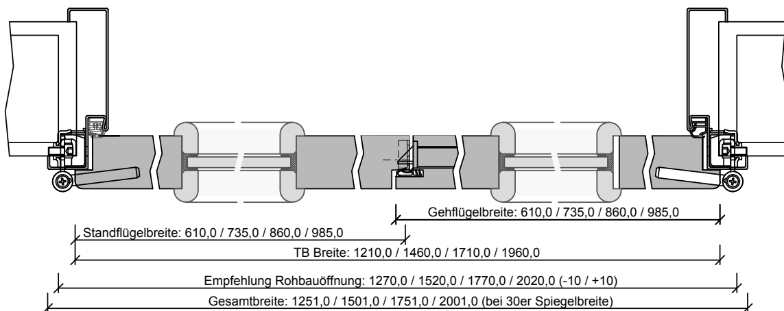
G-Q-SD-TB-SZ-2FLG-SH-GEF-SD-LA.dwg
