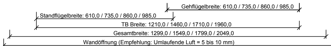
G-Q-SD-TB-BLO-2FLG-SH-GEF-SD-LA.dwg
