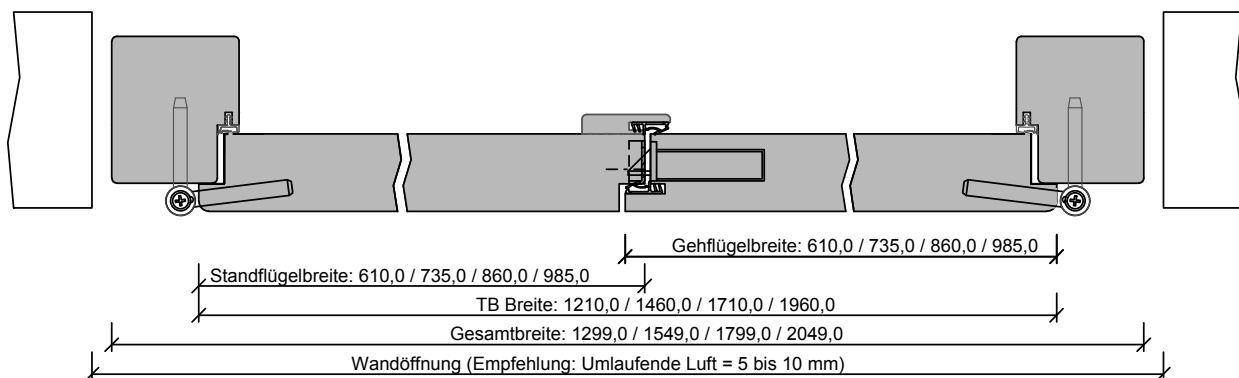
G-Q-SD-TB-BLO-2FLG-SH-GEF-SD-SSK3.dwg
