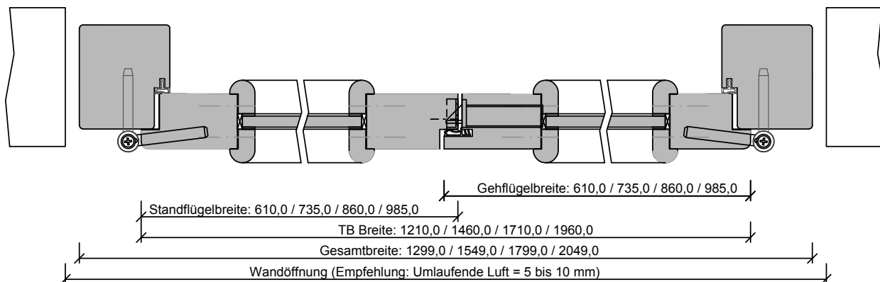
G-Q-SD-TB-BLO-2FLG-SH-GEF-SD-LA.dwg
