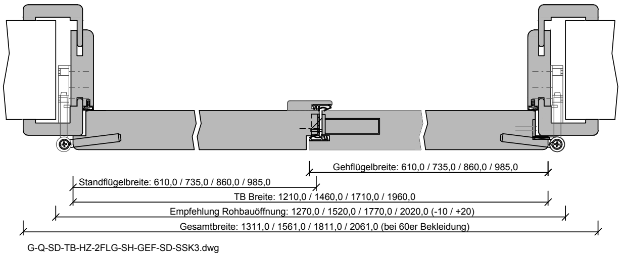
G-Q-SD-TB-HZ-2FLG-SH-GEF-SD-SSK3.dwg
