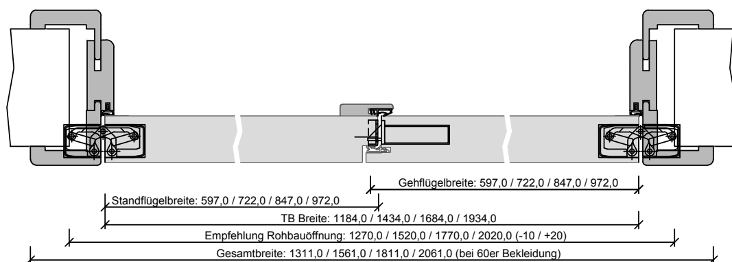
G-Q-SD-TB-HZ-2FLG-SH-STU-SD-SSK3.dwg
