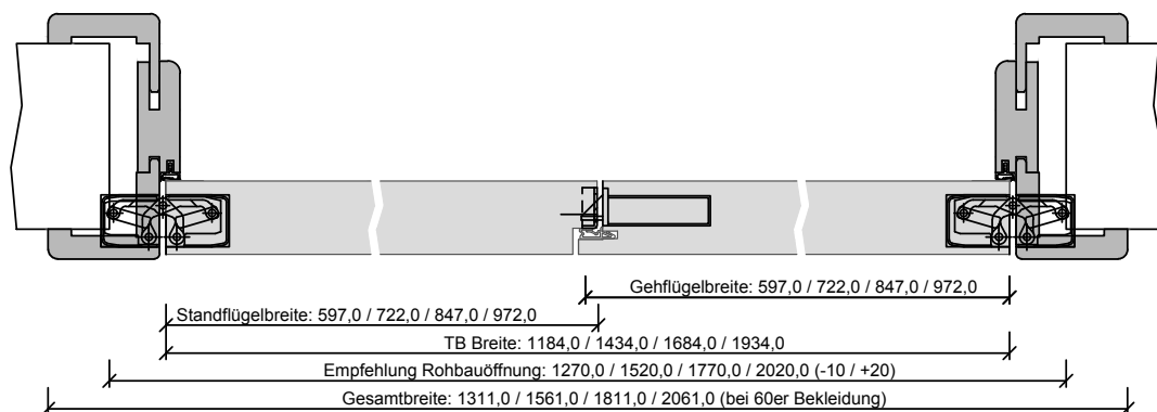
G-Q-SD-TB-HZ-2FLG-SH-STU-SD.dwg
