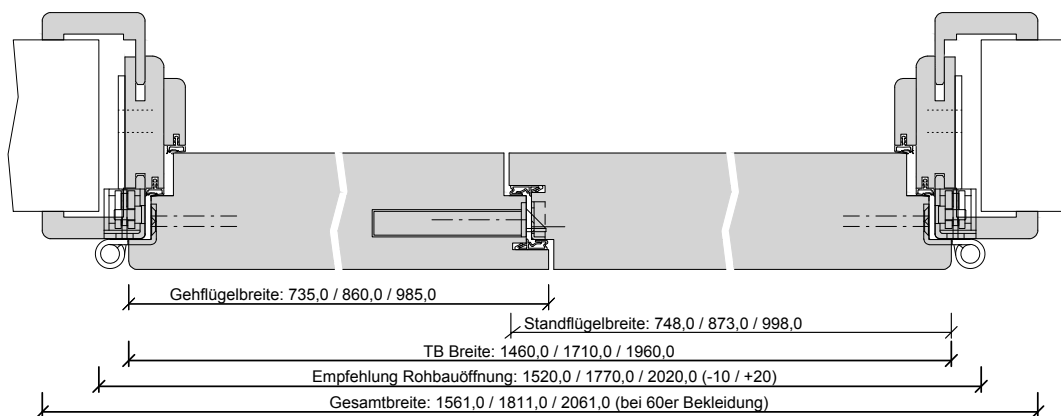
G-Q-SD-TB-HZ-2FLG-SH-GEF-SD-SSK4.dwg
