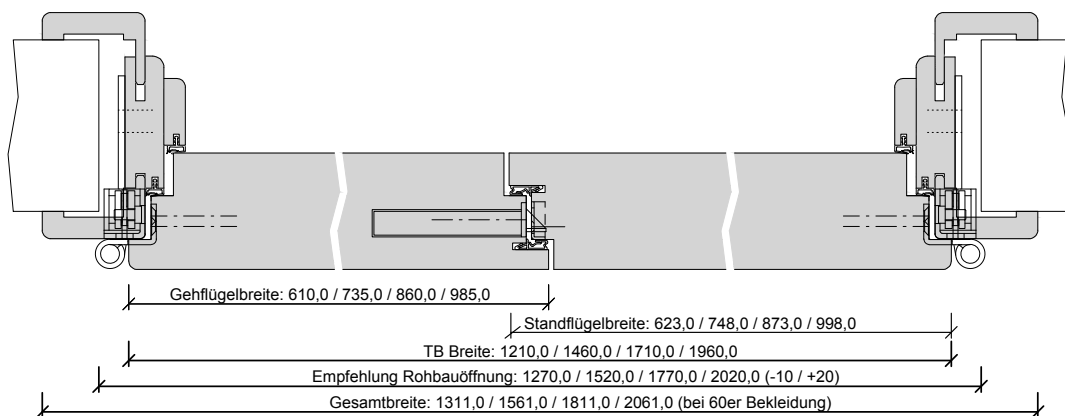
G-Q-SD-TB-HZ-2FLG-SH-GEF-DF-SSK3.dwg
