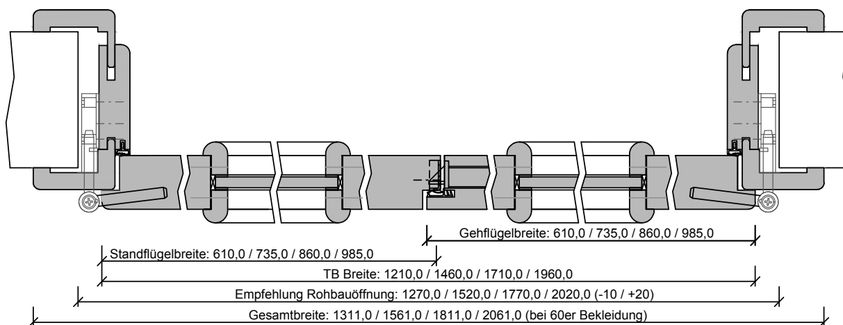
G-Q-SD-TB-HZ-2FLG-SH-GEF-SD-LA.dwg
