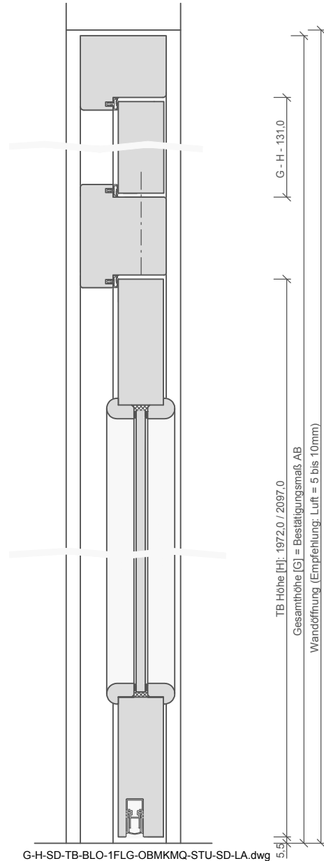
G-H-SD-TB-BLO-1FLG-OBKMQ-STU-SD-LA.dwg
