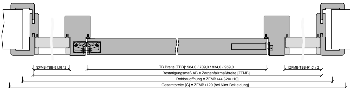
G-Q-SD-TB-HZ-1FLG-WF2-STU-SD-SSK3.dwg
