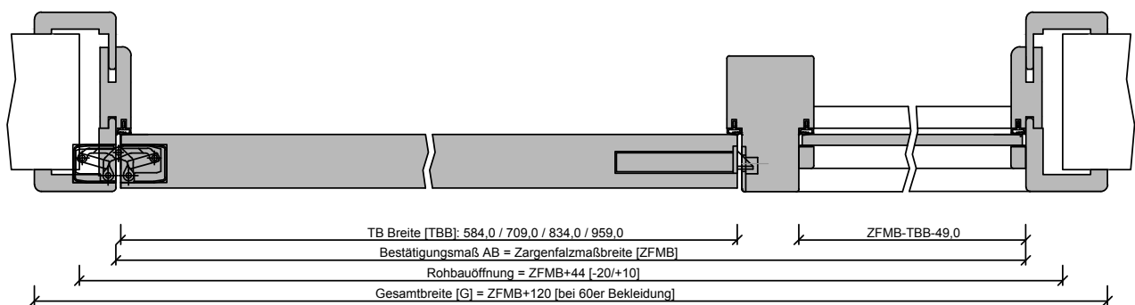
G-Q-SD-TB-HZ-1FLG-WF1-STU-SD.dwg
