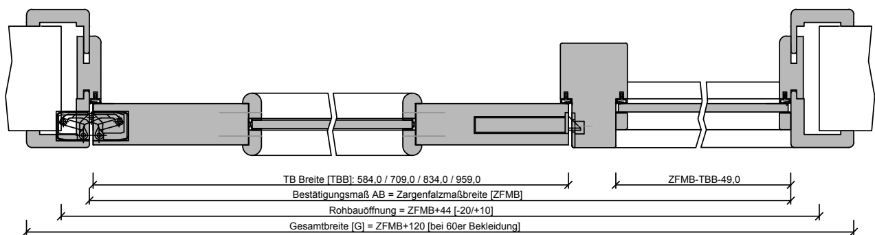
G-Q-SD-TB-HZ-1FLG-WF1-STU-SD-LA.dwg
