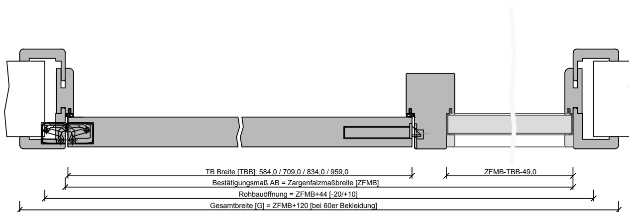
G-Q-SD-TB-HZ-1FLG-WF1-STU-SSK3.dwg
