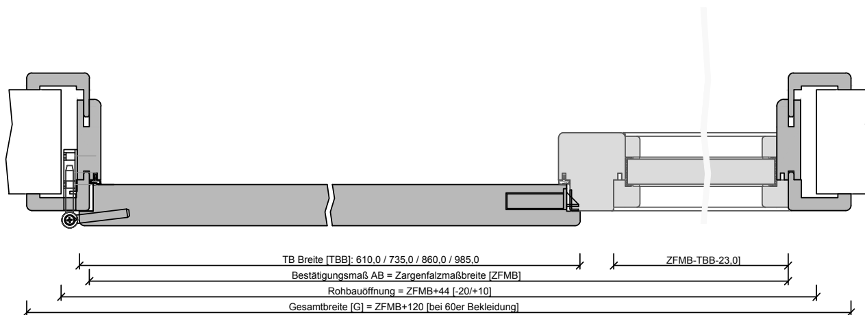
G-Q-SD-TB-HZ-1FLG-WF1-GEF-SD-SSK3.dwg
