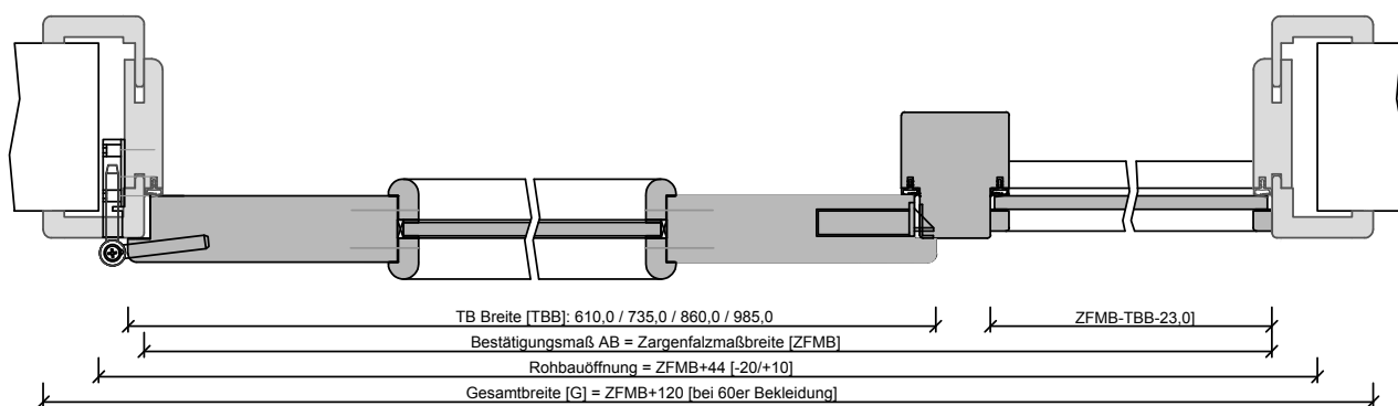
G-Q-SD-TB-HZ-1FLG-WF1-GEF-SD-LA.dwg
